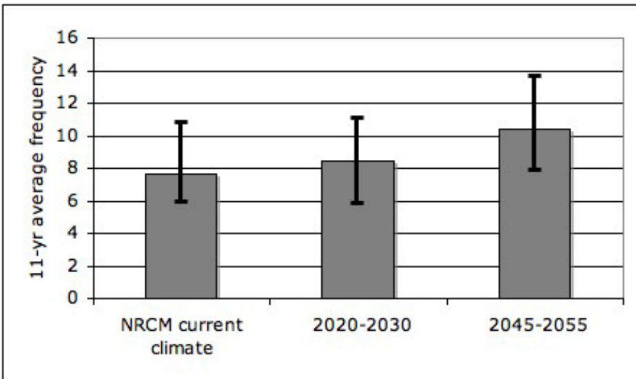
Figure 15: Simulated 11-year average annual tropical cyclone frequency from the 36 km domain using the standard tracking criteria of 17 \text{ m/s} and 2 day duration (gray bars) and the range determined using two tracking criteria combinations representing lenient ( 14.5 \text{ m/s} and 42 hours duration) and strict ( 19.5 \text{ m/s} and 54 hours duration) extremes (black lines).
