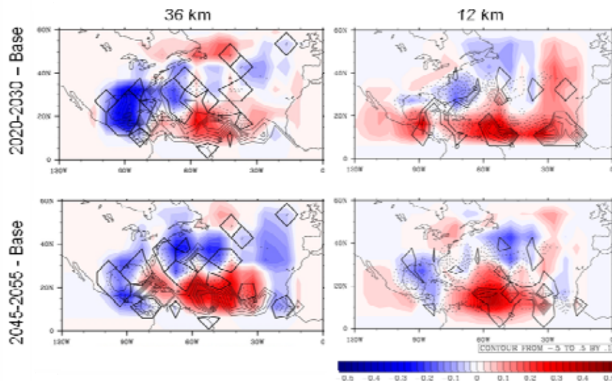
Figure 10: Future change in tropical cyclone track density (colors) and genesis density (contours, positive is solid and negative is dashed) for all NRCM tropical cyclones generated on (left column) the 36 km domain and (right column) the 12 km domain. The change from base climate is (top row) to 2020-2030 and (bottom row) to 2045-2055. The densities represent the number of 6-h occurrences within overlapping 5° Marsden squares, normalized to a maximum value of 1.
