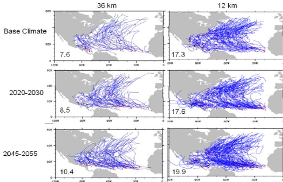
Figure 8: Tropical cyclone genesis points (red) and tracks (blue) for all NRCM tropical cyclones generated on the (left column) 36 km domain and on the (right column) 12 km domain for (top row) base climate, (middle row) 2020-2030, and (bottom row) 2045-2055. The numbers in the bottom left of each panel indicate the average annual tropical cyclone frequency.
